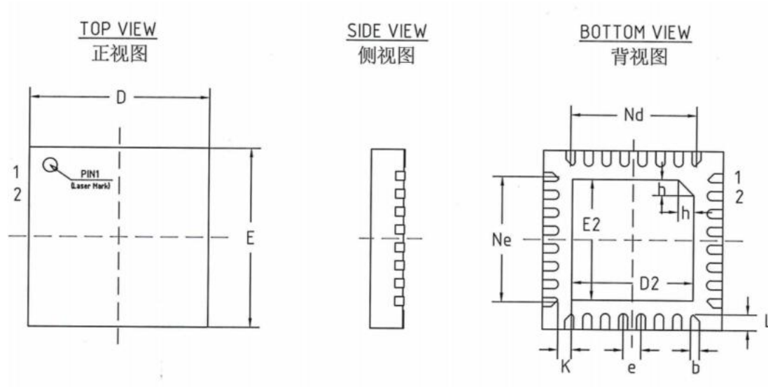
COMMON DIMENSIONS
